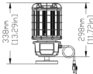
5. Magnetic bracket
