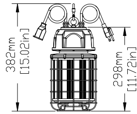
1. Suspension loop
