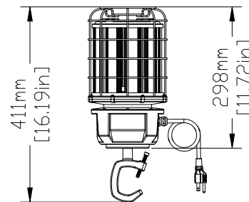
4. U clamp
